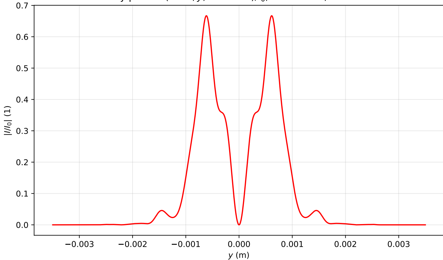
Intensity profile I(x=0, y, z=1.592)/I_0 , P_{in}=6.0P_{cr} , artificial time
